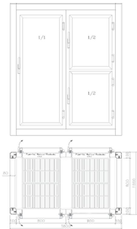
AMD/P 1803 [Puertas a ambas caras] 1000x1800x80 Ht: 2120 [+]
